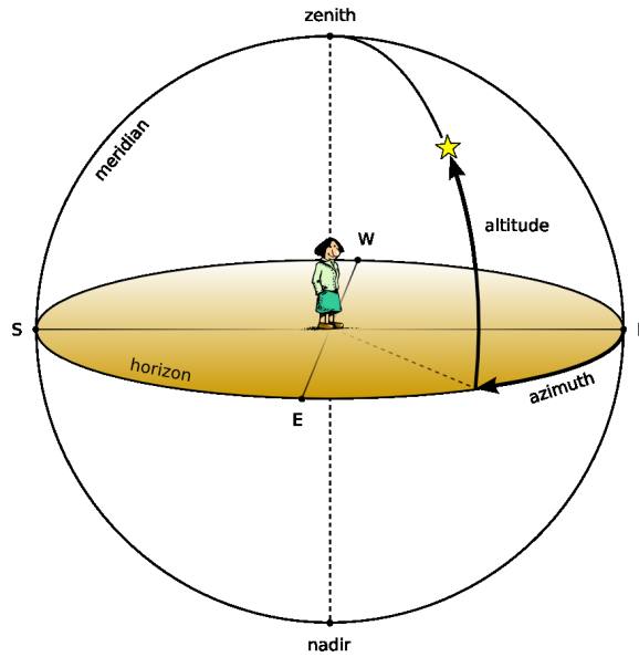
Figure F.1: Altitude & Azimuth
