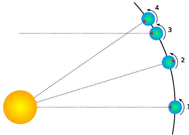
Figure F.3: Solar and Sidereal days
