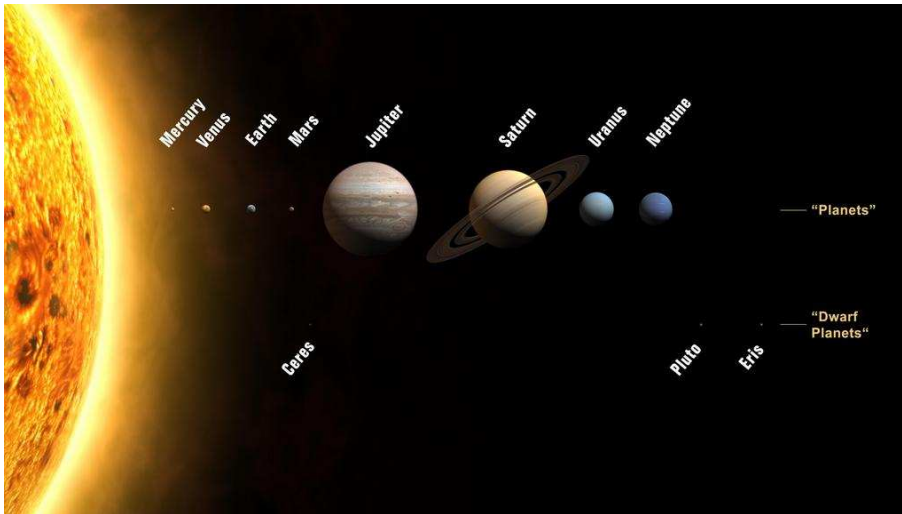
Figure G.4: Planets and dwarf planets in our solar system. The planet sizes are drawn to scale, but not their distances from the Sun or one another.
