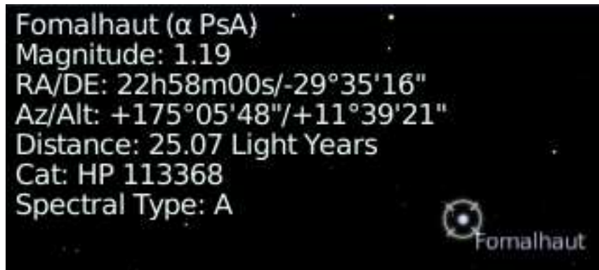
Figure G.2: Stellarium displaying information about a star
