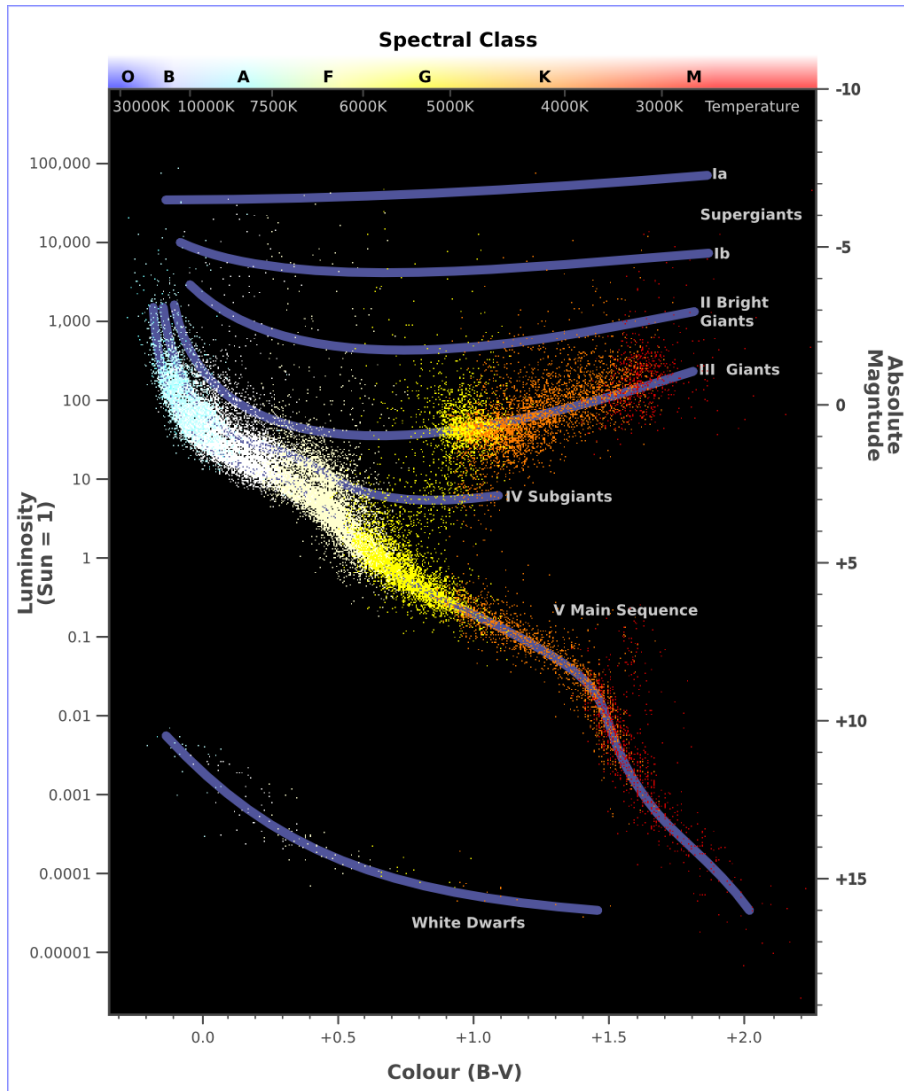
Figure G.3: Plot of star colour vs. magnitude
