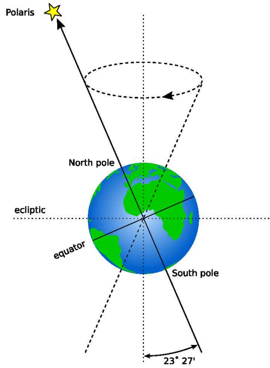
Figure F.5: Precession
