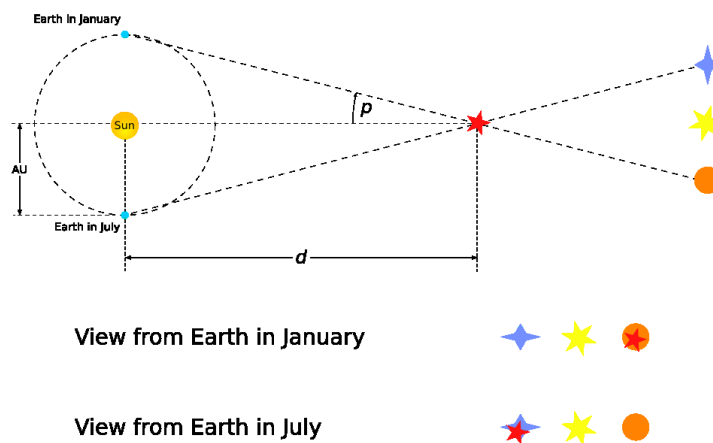
Figure F.6: Apparent motion due to parallax
