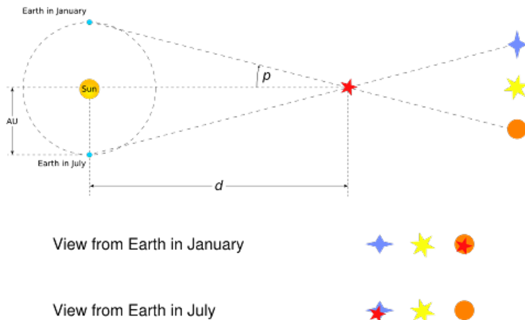
Figure 17.7: Stellar Parallax
