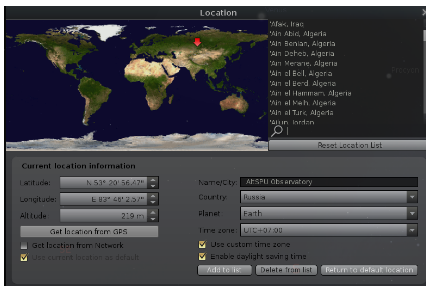
Figure 4.2: Location window
