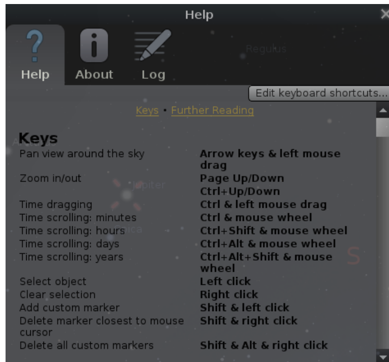
Figure 4.31: Help Window
