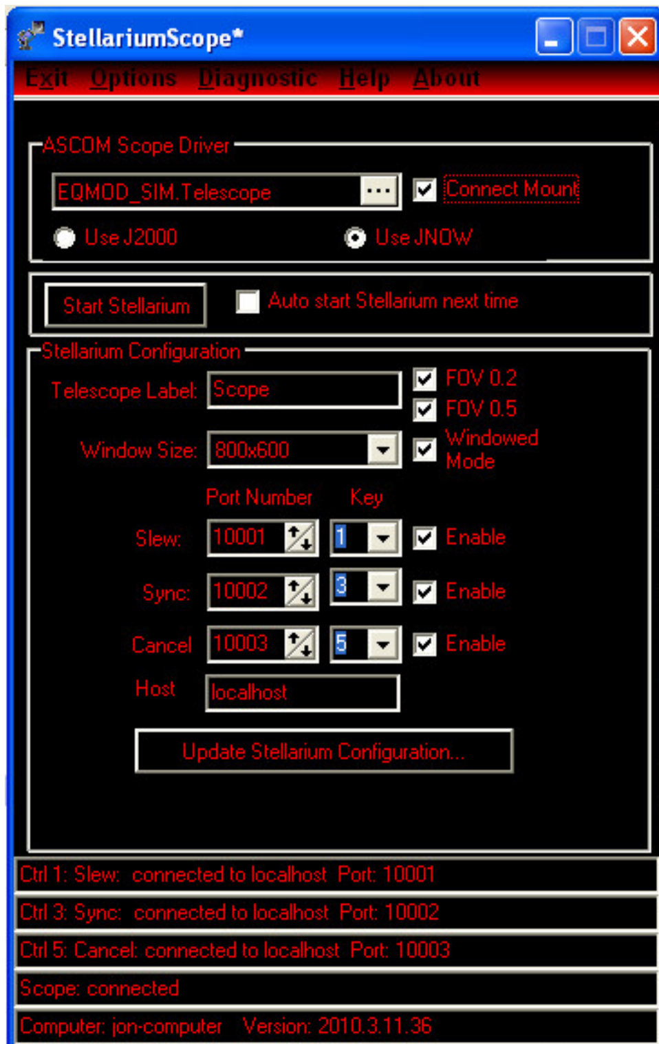
Figure 15.18: StellariumScope interface
