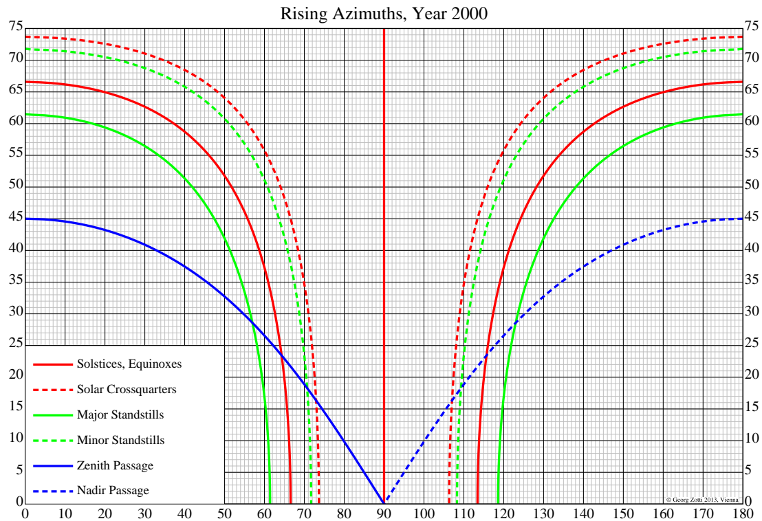
Figure 13.12: Rising azimuths of a few important events for sun and moon, and zenith and nadir passages depending on geographic latitudes (vertical axis).
