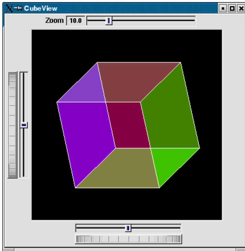
Figure 9-2: CubeView demo.
