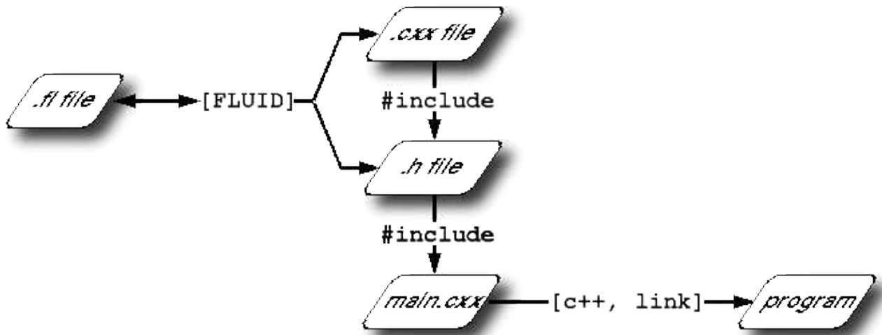
Figure 9-1: FLUID organization.
