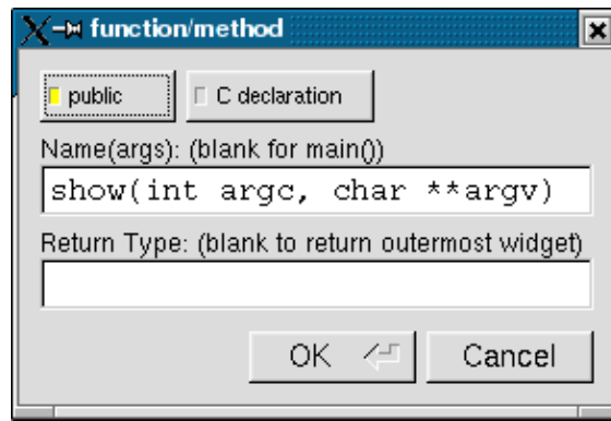
Figure 9-6: CubeView constructor.
