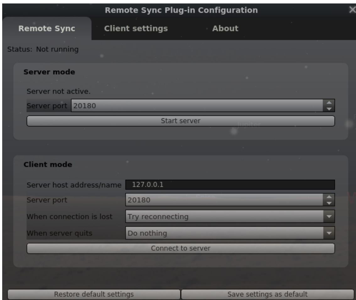
Figure 13.4: RemoteSync settings window
