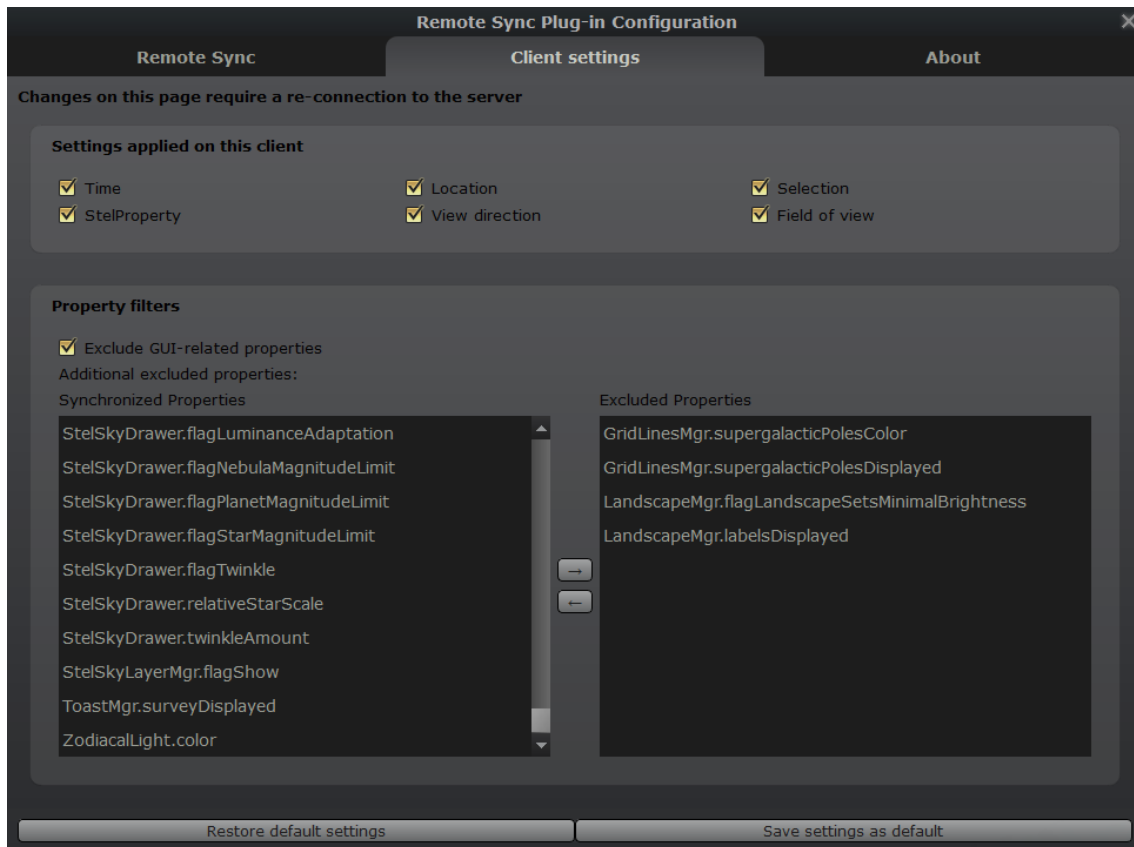
Figure 13.5: RemoteSync client settings window
