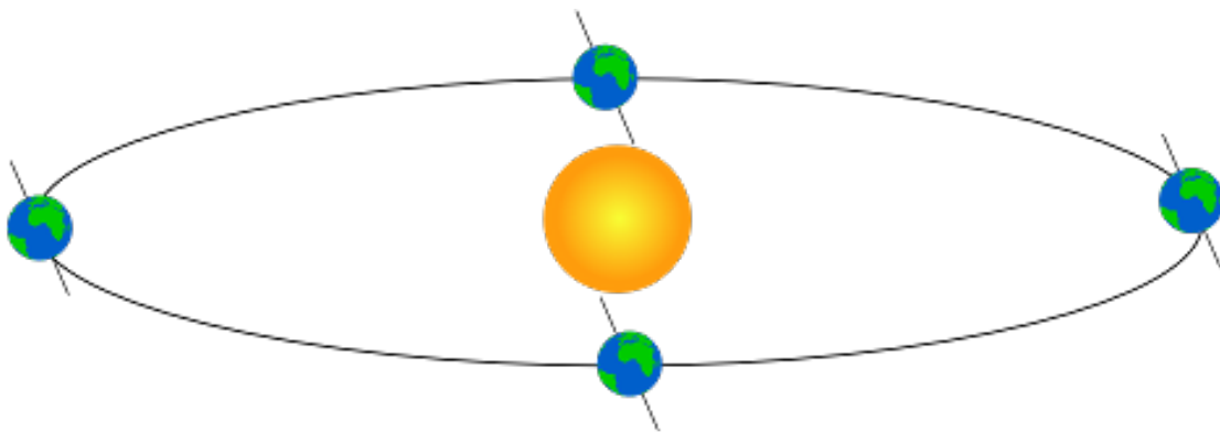
Figure 18.4: Ecliptic obliquity
