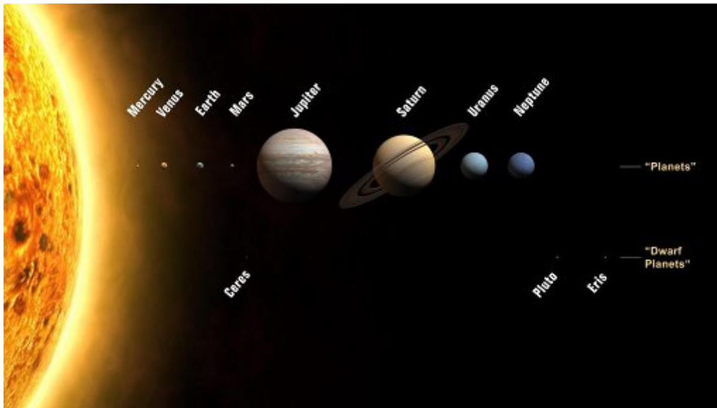
Figure 19.4: The Planets
