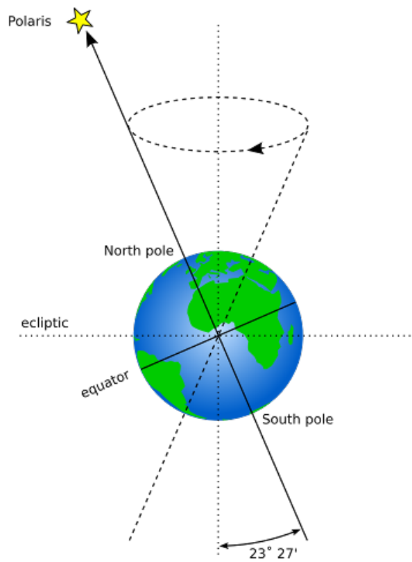
Figure 18.5: Precession
