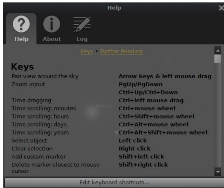
Figure 4.45: Help Window
