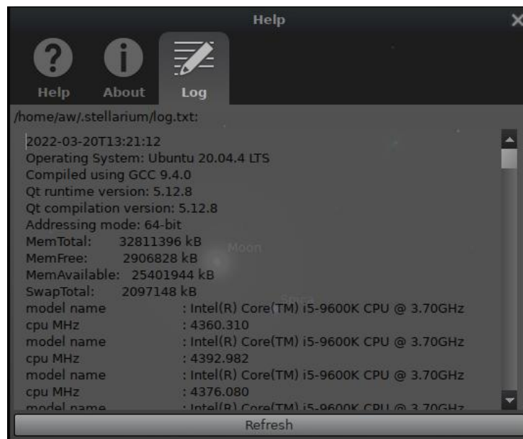
Figure 4.47: Help Window: Logfile
