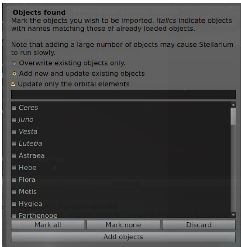
Figure 13.9: Interface of Solar System Editor plugin: Import data dialog — view after downloading and parsing the MPC data.
