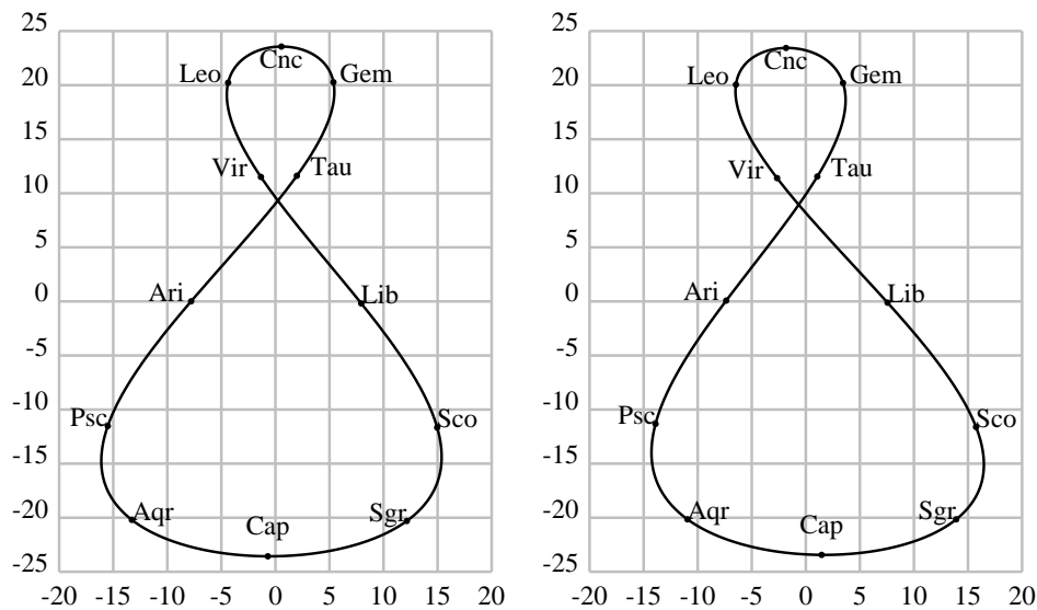
Figure 13.1: Figure-8 plots for Equation of Time, for years 1000 (left) and 2000 (right). These plots, often found on sundials, link solar declination (vertical axis) and its deviation at mean noon from the meridian, in minutes. Labeled dots indicate when the sun entered the respective Zodiacal sign ( 30^\circ section of the ecliptic). Figures by Georg Zotti.
