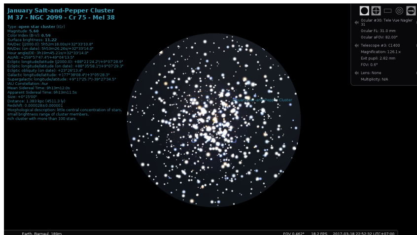
Figure 16.10: The M37 cluster through a Celestron C1400 with Tele Vue Nagler 31 mm eyepiece.
