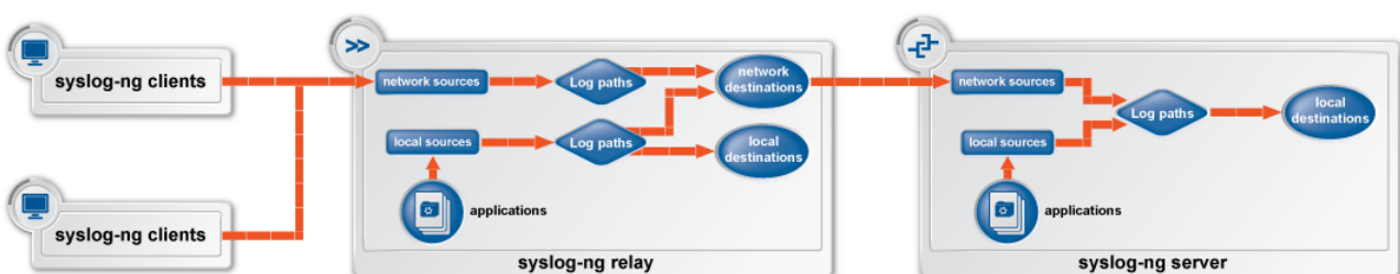
Figure 2.5. Relay-mode operation
